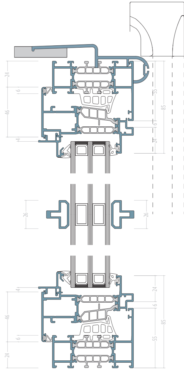
Rollladentraverse
